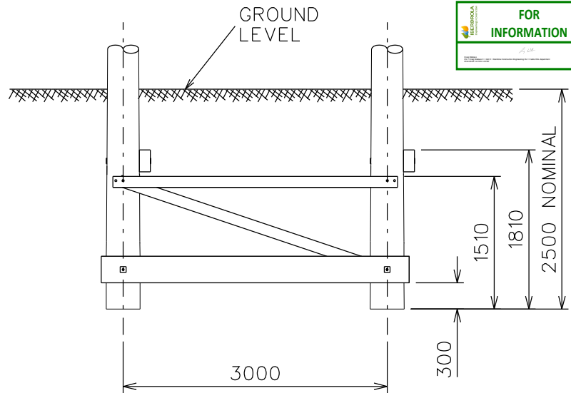
14M POLE FRONT ELEVATION
